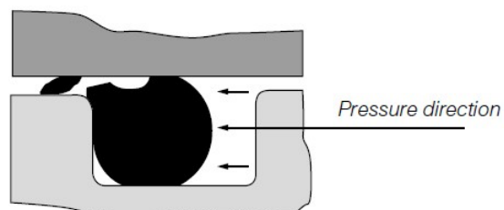
Extruded O-Ring
