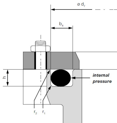
Flange seal – internal pressure
